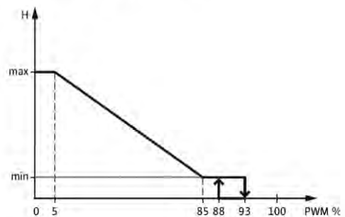
PWM signal logic (heating):
